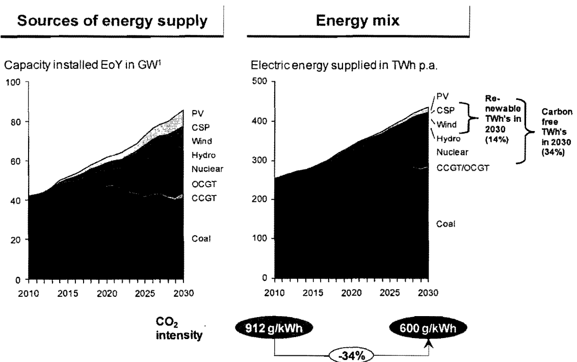
Figure 8. Capacity and energy mix 2010-2030
