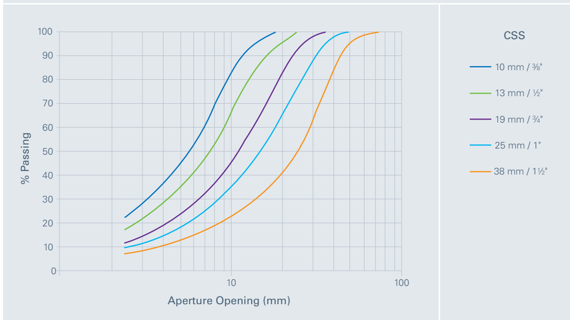
Trio® TP Cone Crusher Gradation Curves
