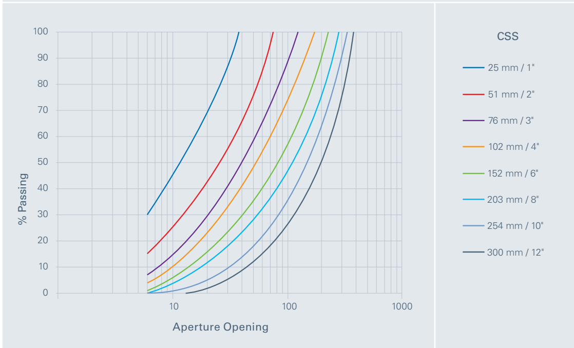
Trio® CT Jaw Crusher Gradation Curves
