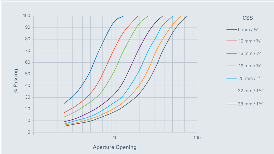
Trio® TC Cone Crusher Gradation Curves
